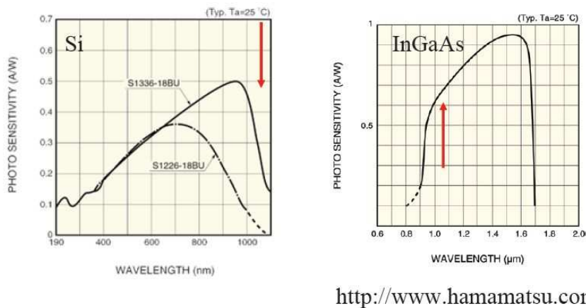
FIG. 11: Exemplary sensitivities of Si and InGaAs diodes.
