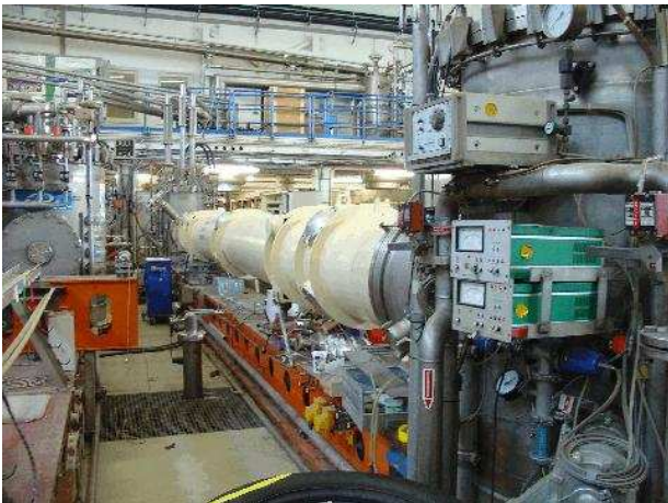
FIG. 5: HERA dipole at the magnet test stand.
