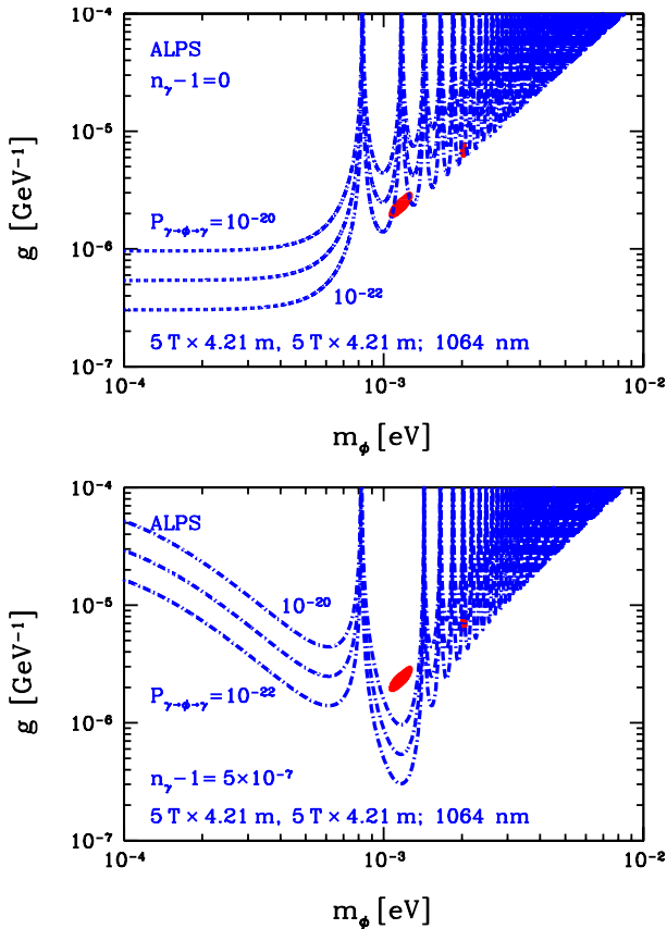
FIG. 3: Two photon coupling g of the (pseudo-)scalar versus its mass m_\phi . The 3 sigma allowed region from PVLAS data on rotation plus BFRT data on rotation, ellipticity, and regeneration is shown in red [8].
